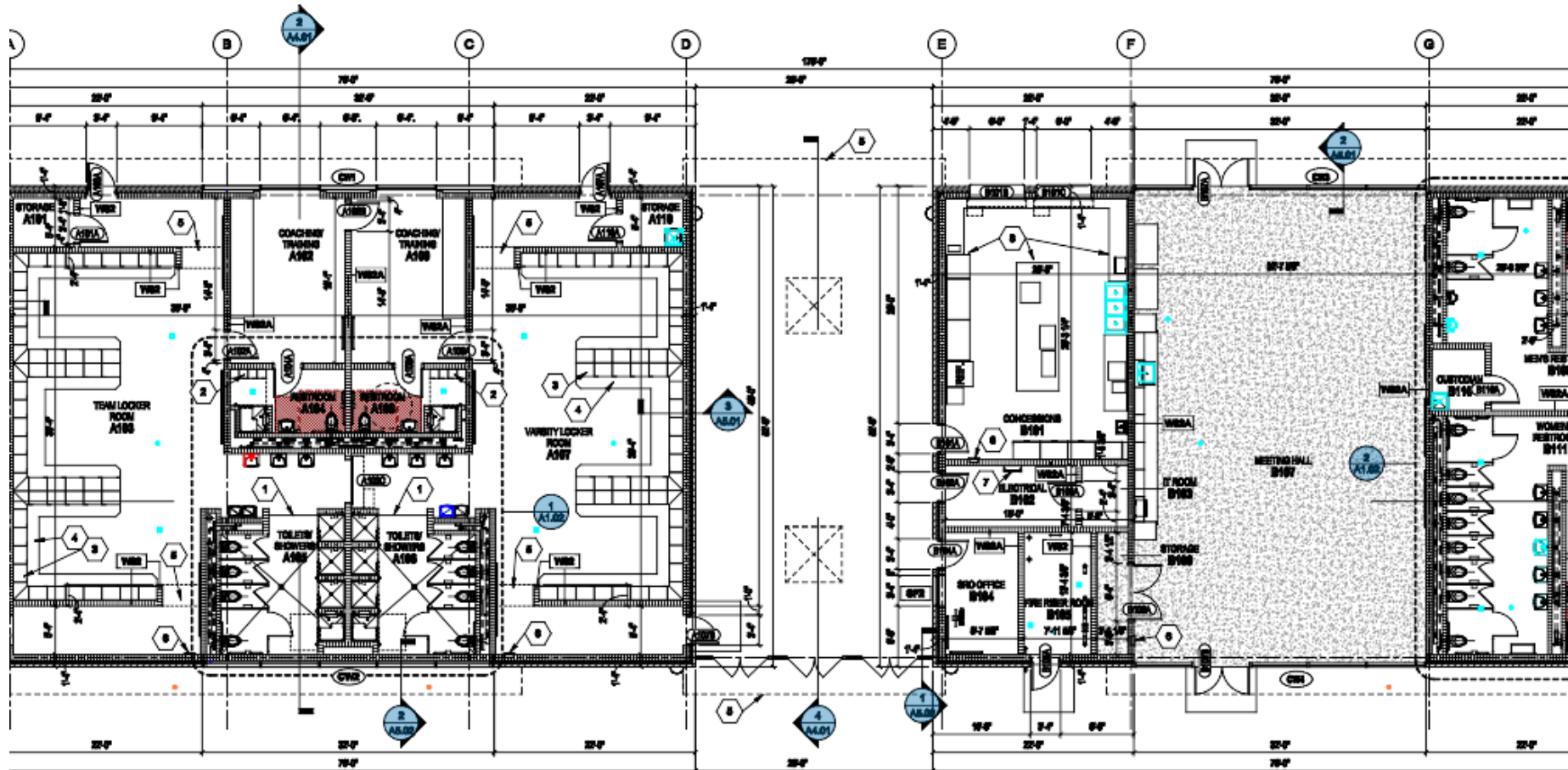
FIRST FLOOR ARCHITECTURAL PLAN
