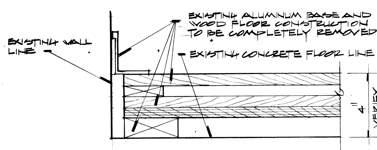
EXISTING GYMNASIUM FLOOR CONSTRUCTION SCALE: 3/8"=1'-0" (VERIFY ALL EXISTING DIMENSIONS & CONDITIONS)
