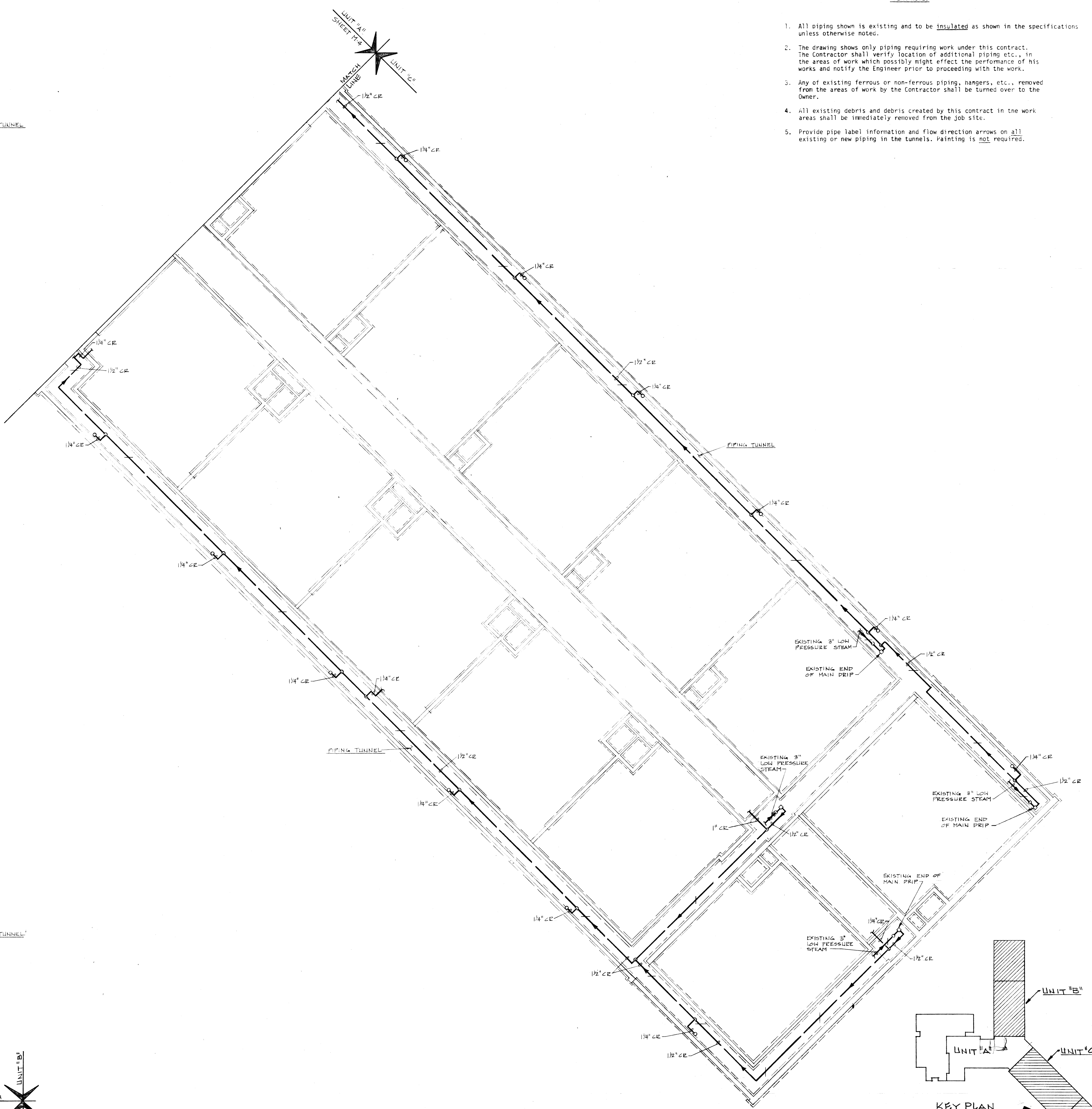
UNIT "C" MECHANICAL FOUNDATION PLAN SCALE: 1/8"=1'-0"
