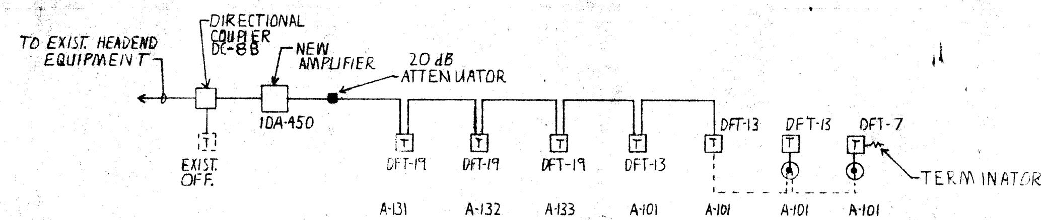
TELEVISION DISTRIBUTION DIAGRAM N.T.S.
