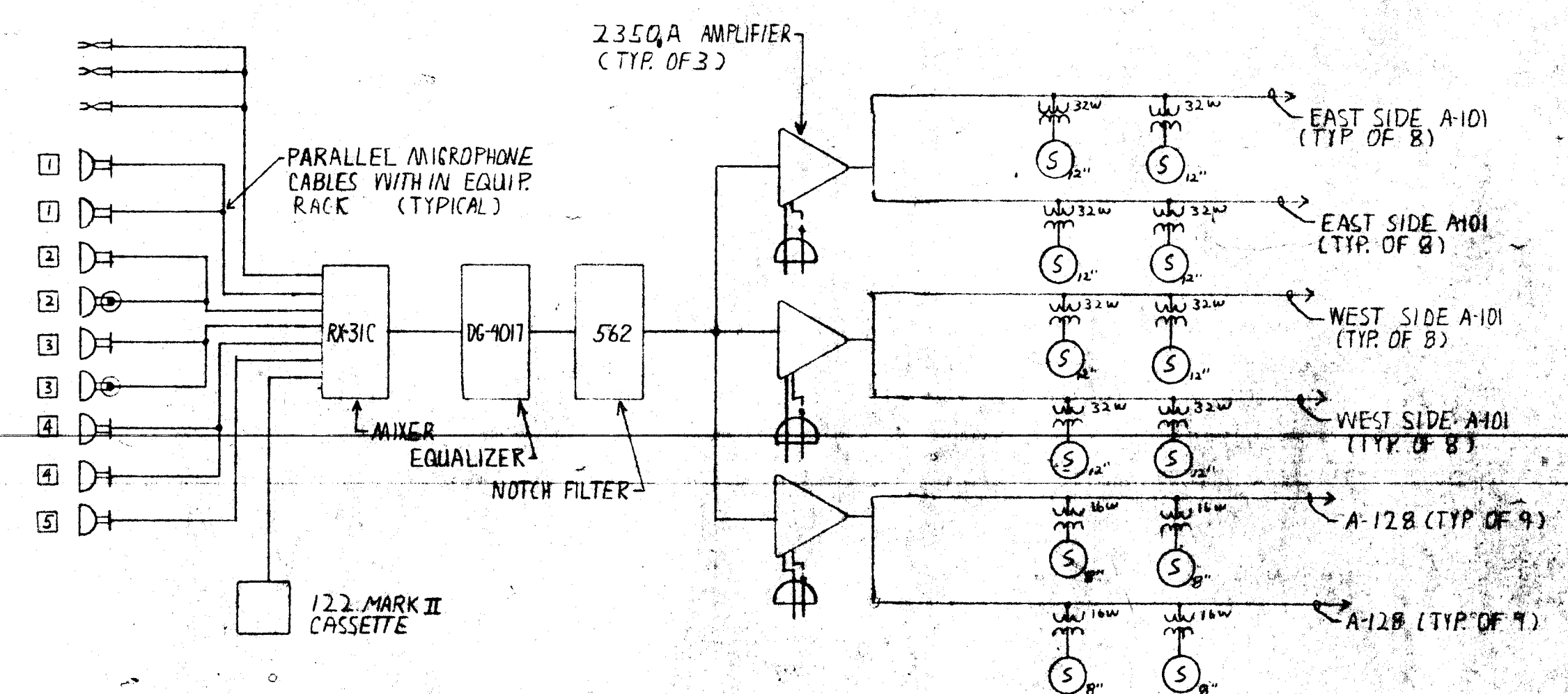
SOUND DISTRIBUTION DIAGRAM N.T.S.
