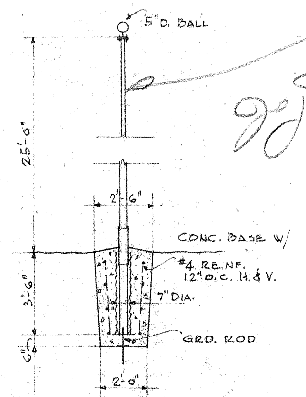
FLAGPOLE DETAIL SCALE 1/4" = 1'-0"
