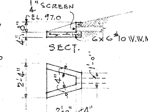
CONCRETE SPLASH PAD SCALE 1/4" = 1'-0"
