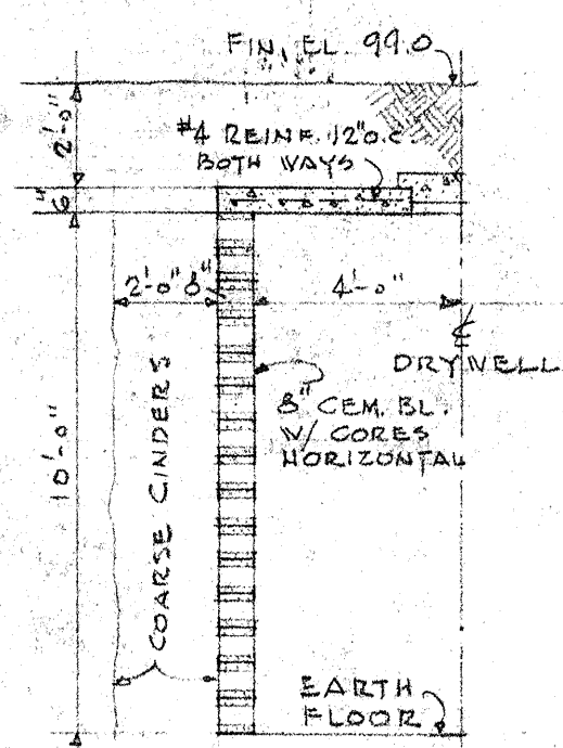
SECTION OF DRYWELL SCALE 1/4" = 1'-0"
