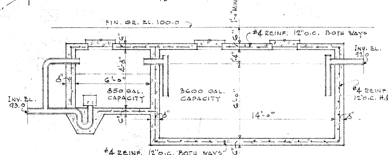
SEPTIC TANK & SIPHON SCALE 1/4" = 1'-0"
