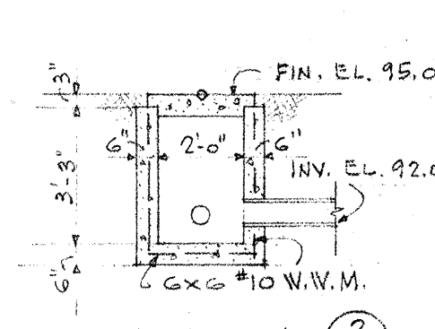
SECTION DISTRIBUTION BOX SCALE 1/4" = 1'-0"
