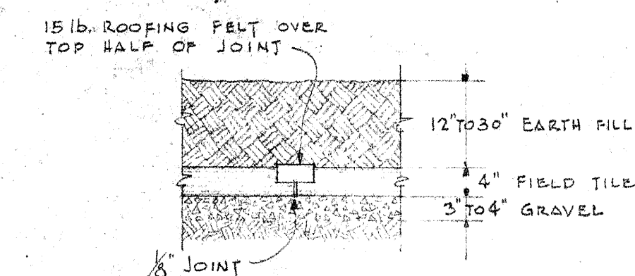
TYPICAL TILE FIELD JOINT DET. SCALE 1/4" = 1'-0"
