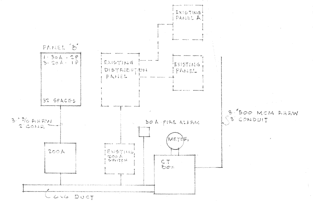
ELECTRICAL SERVICE
