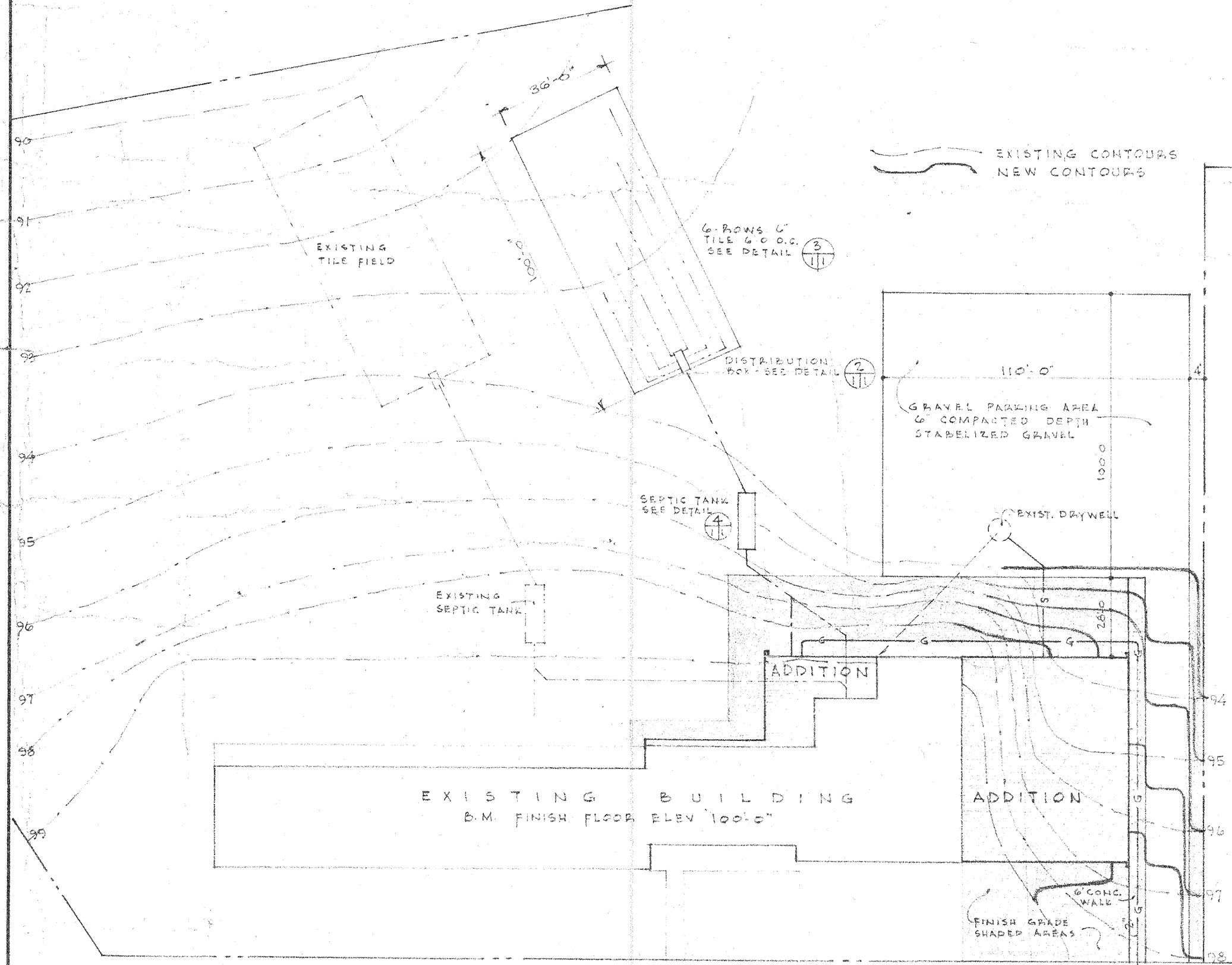
SEPTIC TANK
