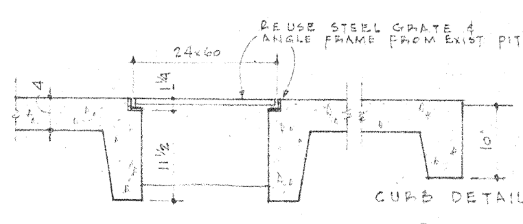
SCRAPE PIT
