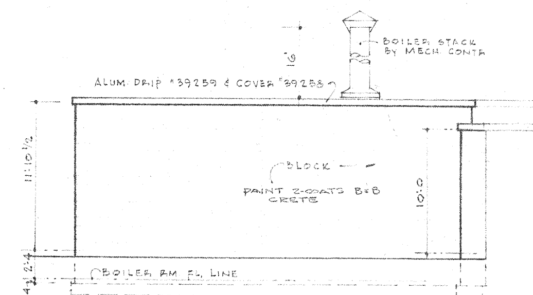
SOUTH ELEVATION 1/8" = 1'-0"
