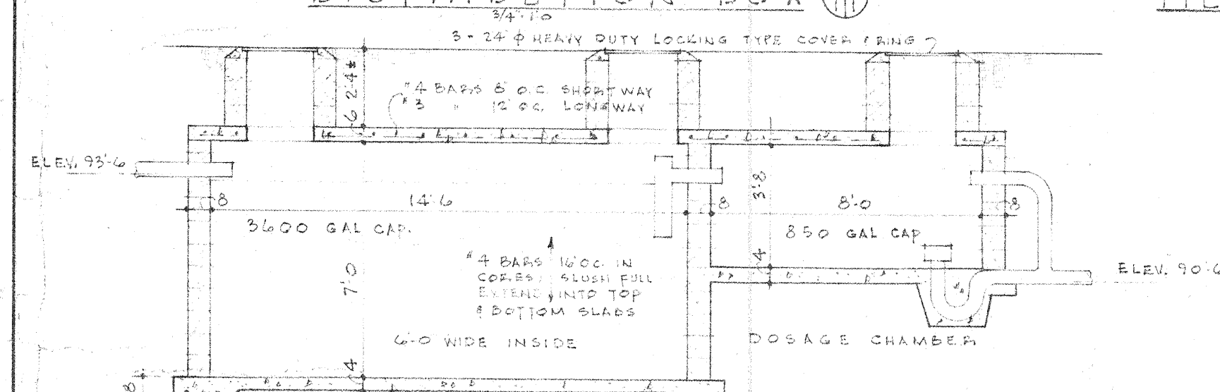
SEPTIC TANK
