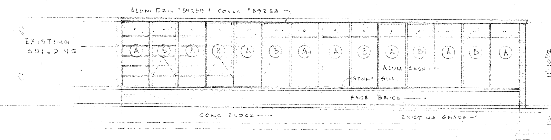
EAST ELEVATION 1/8" = 1'-0"
