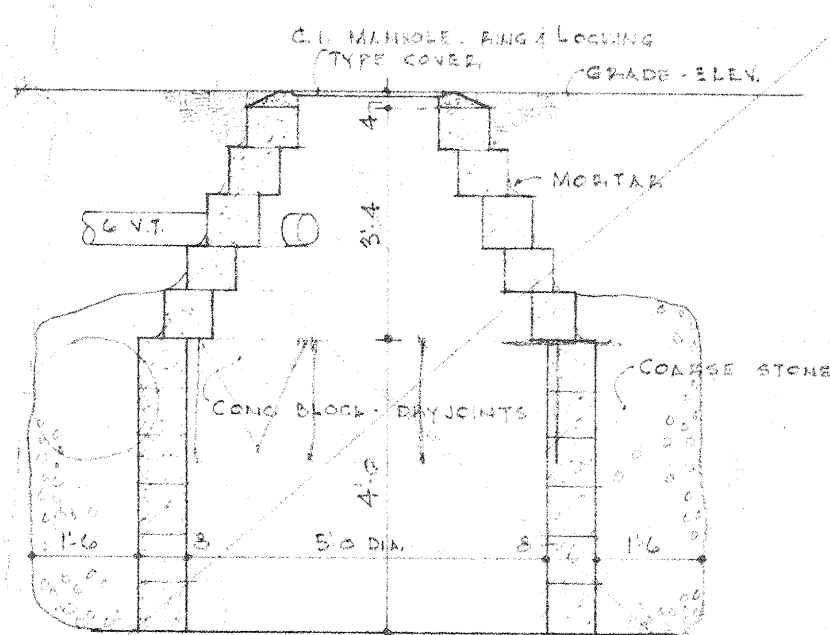
DRYWELL DETAIL BY GEN. CONTR.
